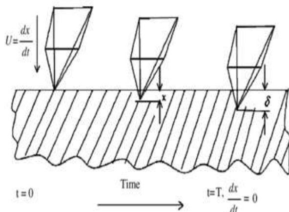
Fig. 4. Scheme of material removal mechanism.
