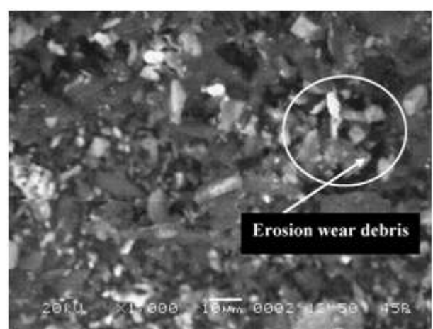
Fig. 2. SEM image of the eroded surface of glass-polyester SiC hybrid composite showing fiber and matrix micro-flake debris.
